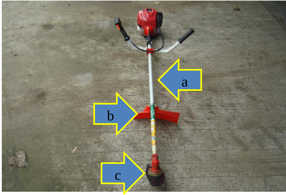
Figure 2. Drive shaft (a), deflector (b) and cutting blade (c)
